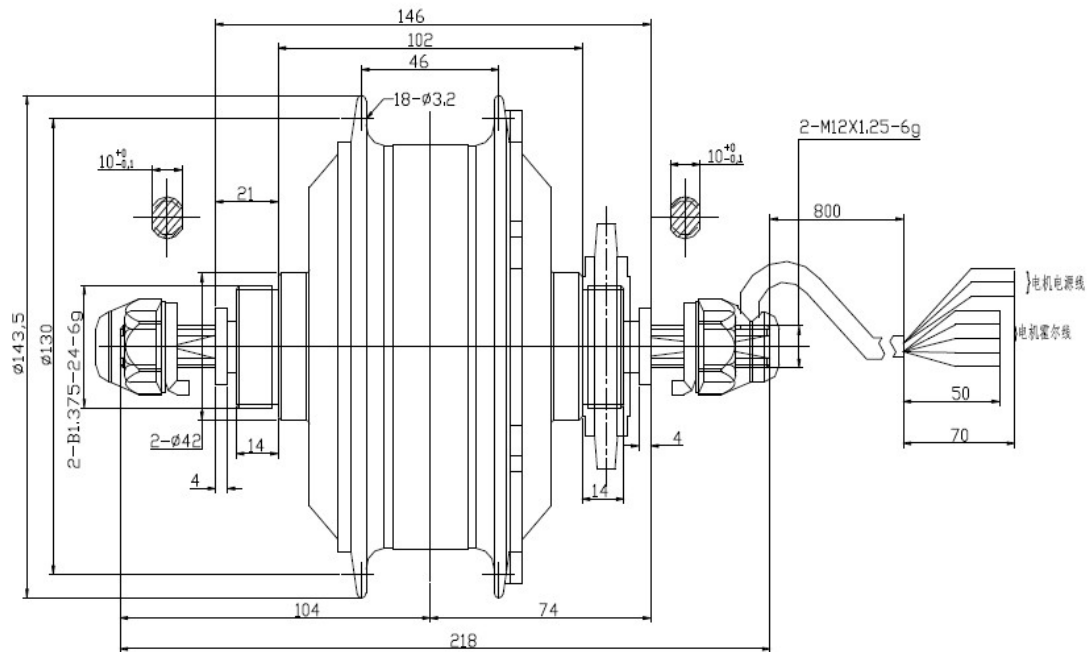
Diagram 3 Rear Motor
