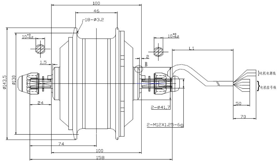
Diagram 2 Front Motor
